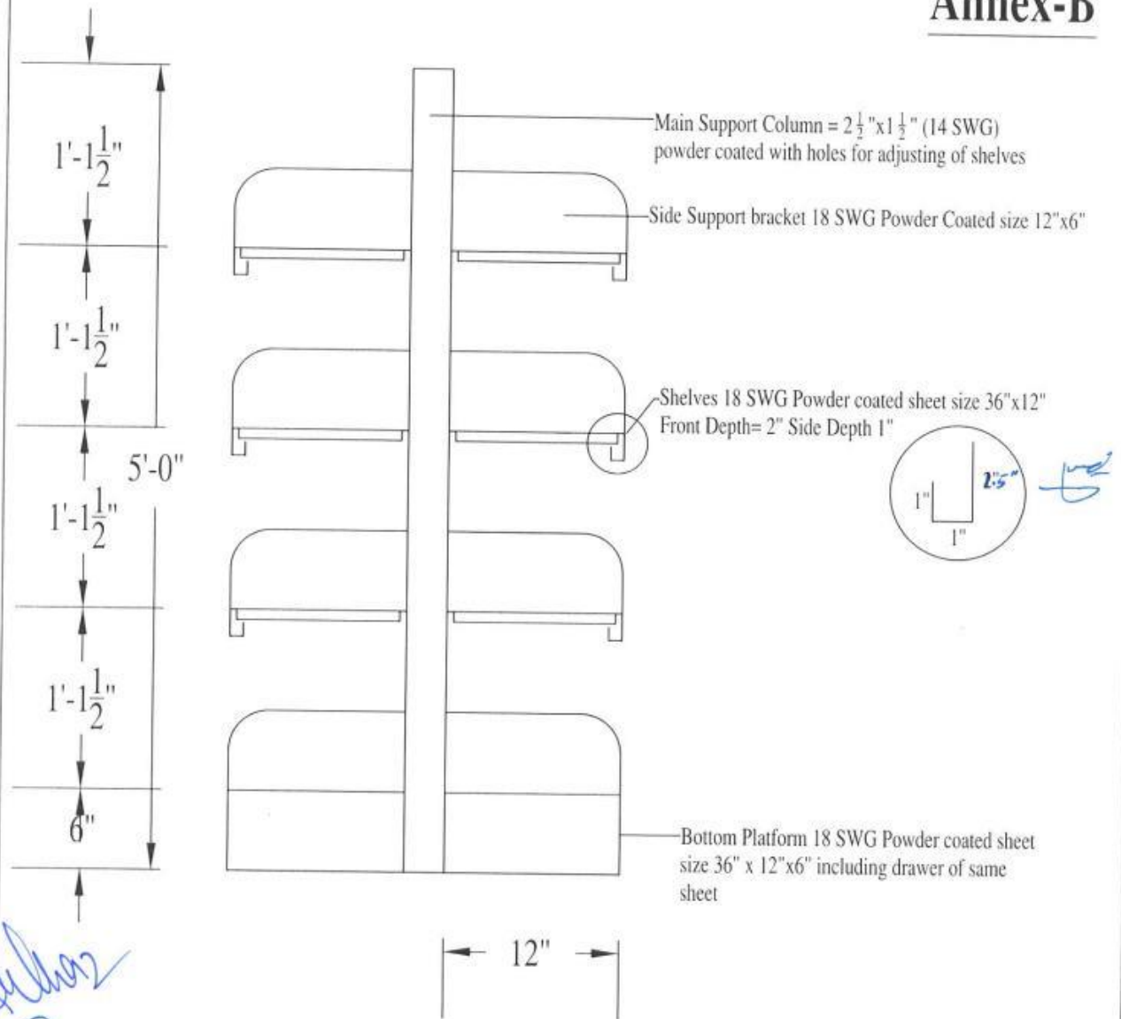
Section of Library Rack size 3ft x 5ft
